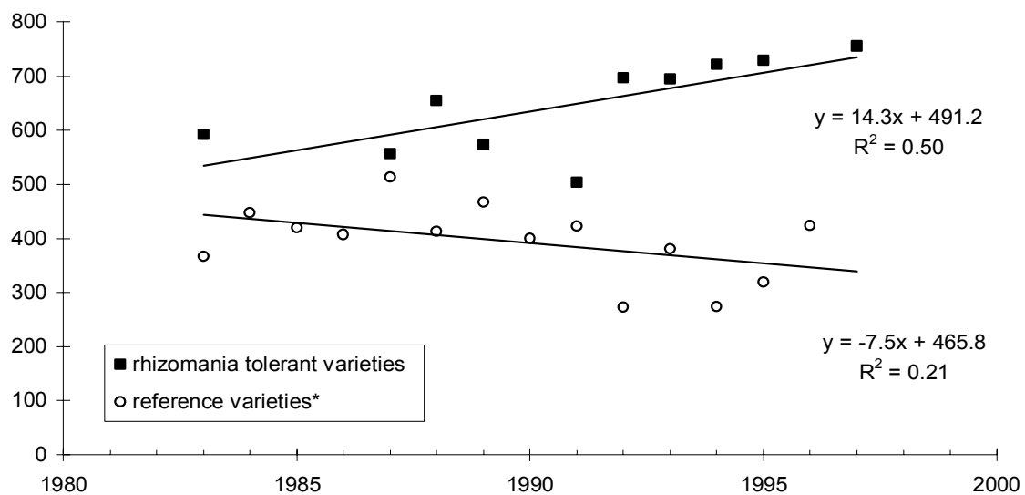
Figure 2: Development of the variety performance of sugar beets in rhizomania infested areas: sugar beet yield [dt/ha]; with x_{1980} = 0
